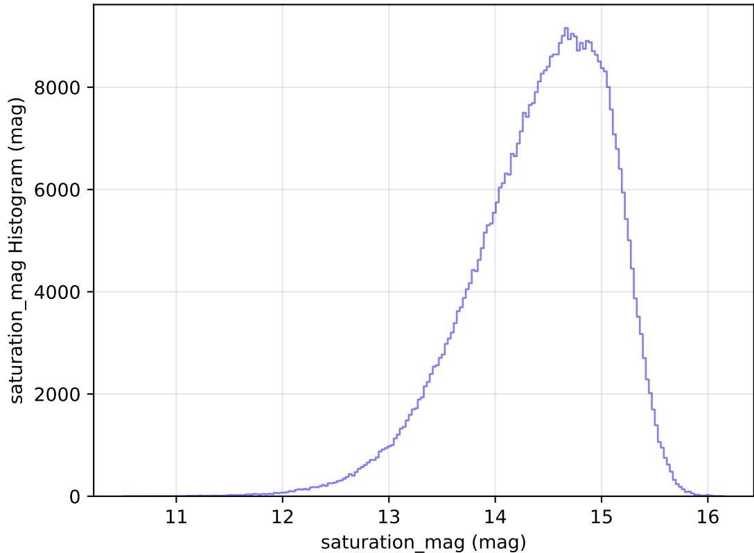
internal_u_expt30_nscale1.1v3.4_10yrs All sky i band: saturation_mag Histogram
