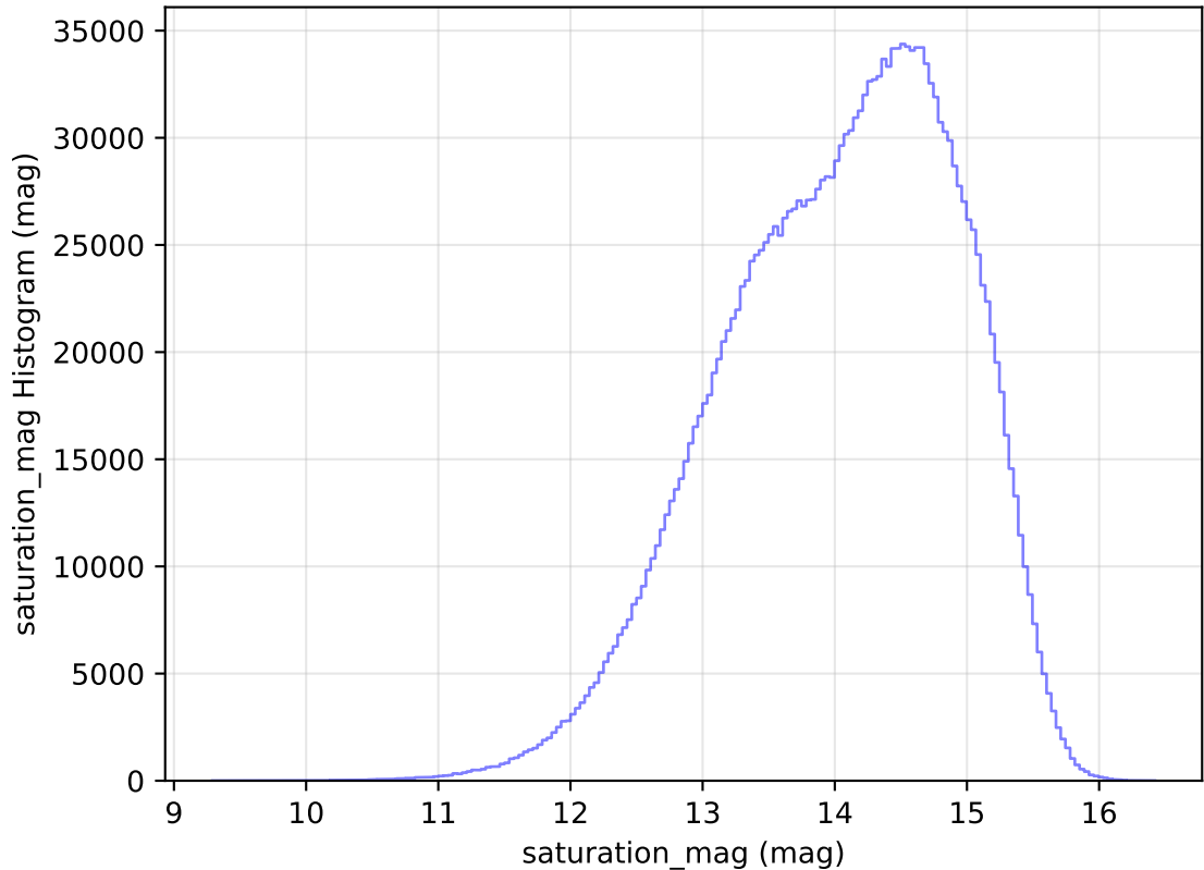
internal_u_expt30_nscale1.1v3.4_10yrs All sky all bands: saturation_mag Histogram
