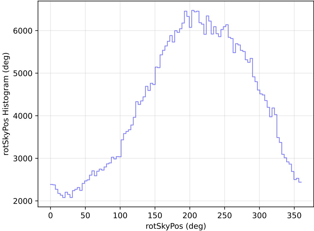
internal_u_expt30_nscale1.1v3.4_10yrs WFD z band: rotSkyPos Histogram
