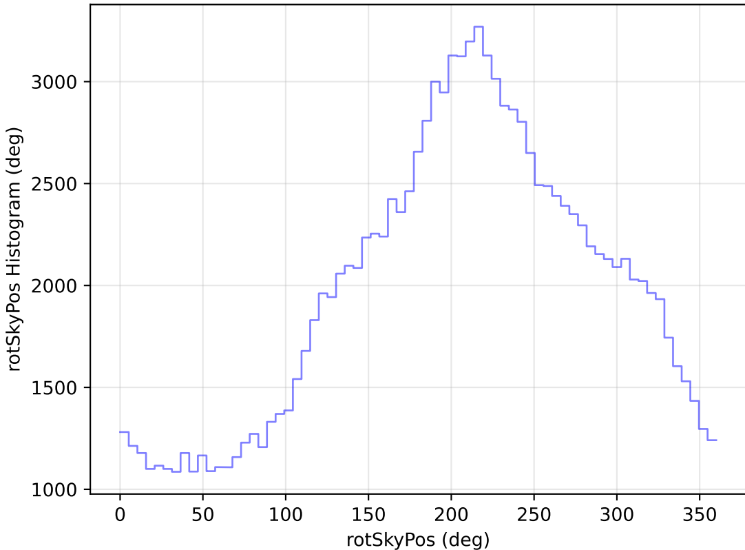
internal_u_expt30_nscale1.1v3.4_10yrs WFD u band: rotSkyPos Histogram
