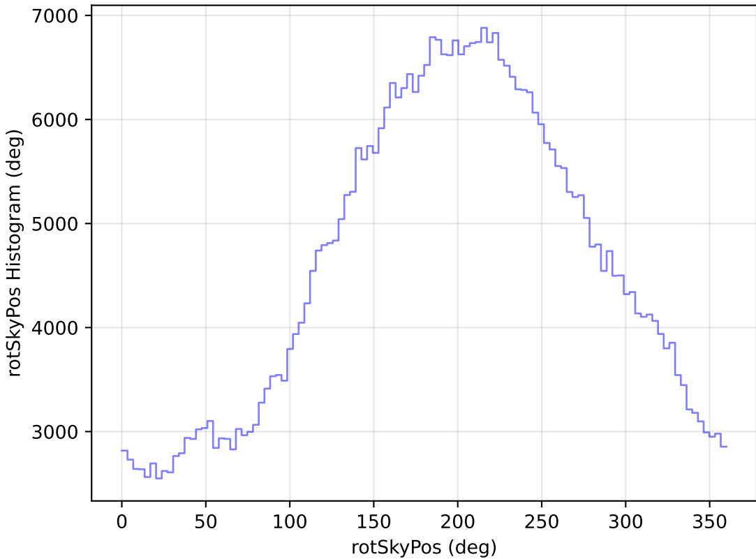
internal_u_expt30_nscale1.1v3.4_10yrs WFD r band: rotSkyPos Histogram
