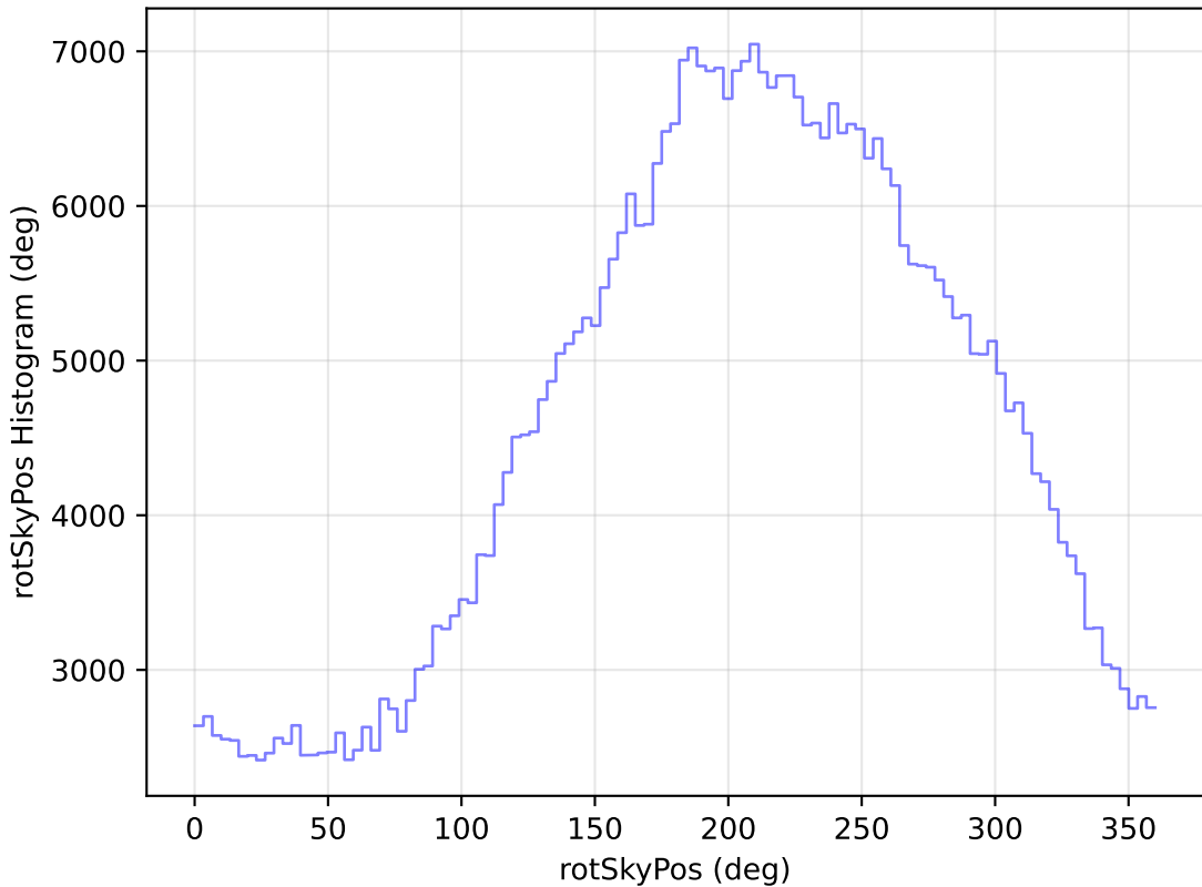
internal_u_expt30_nscale1.1v3.4_10yrs WFD i band: rotSkyPos Histogram
