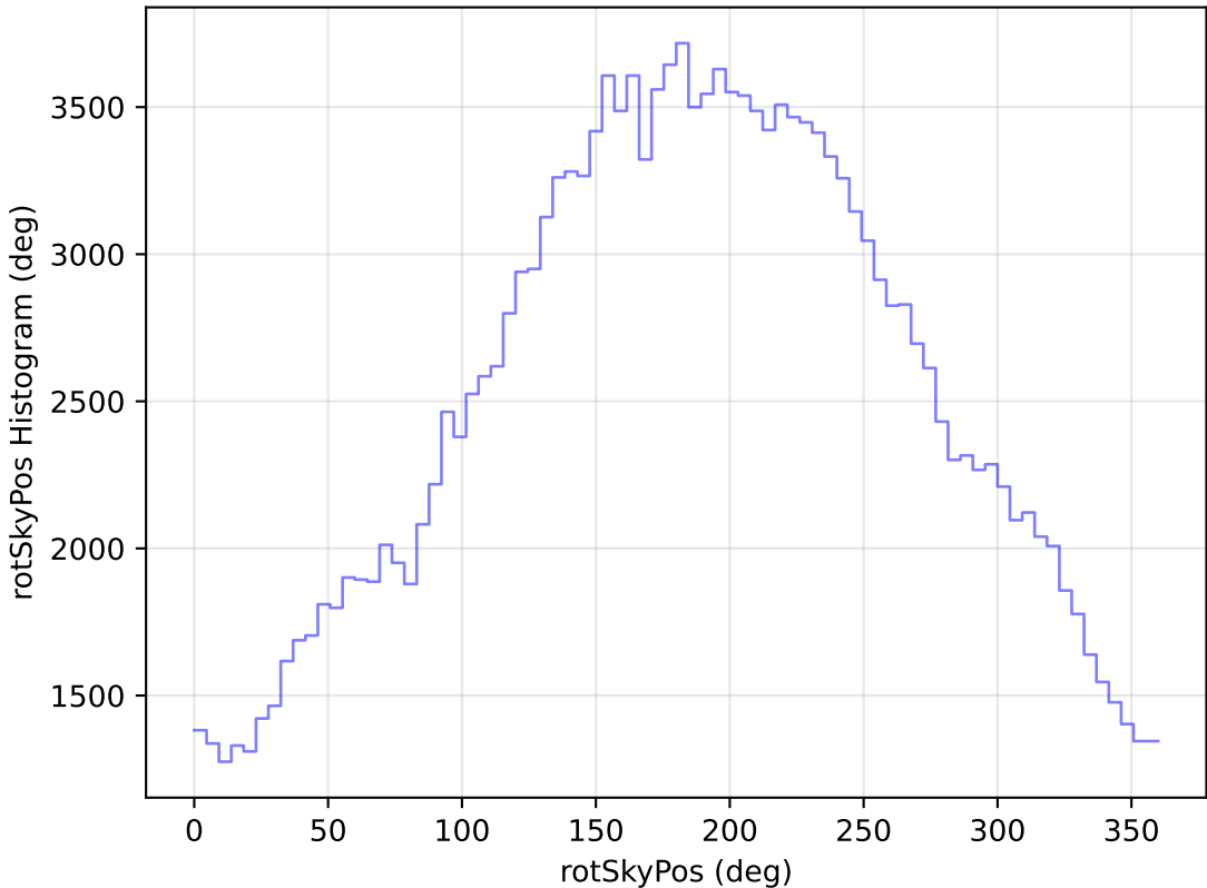
internal_u_expt30_nscale1.1v3.4_10yrs WFD g band: rotSkyPos Histogram
