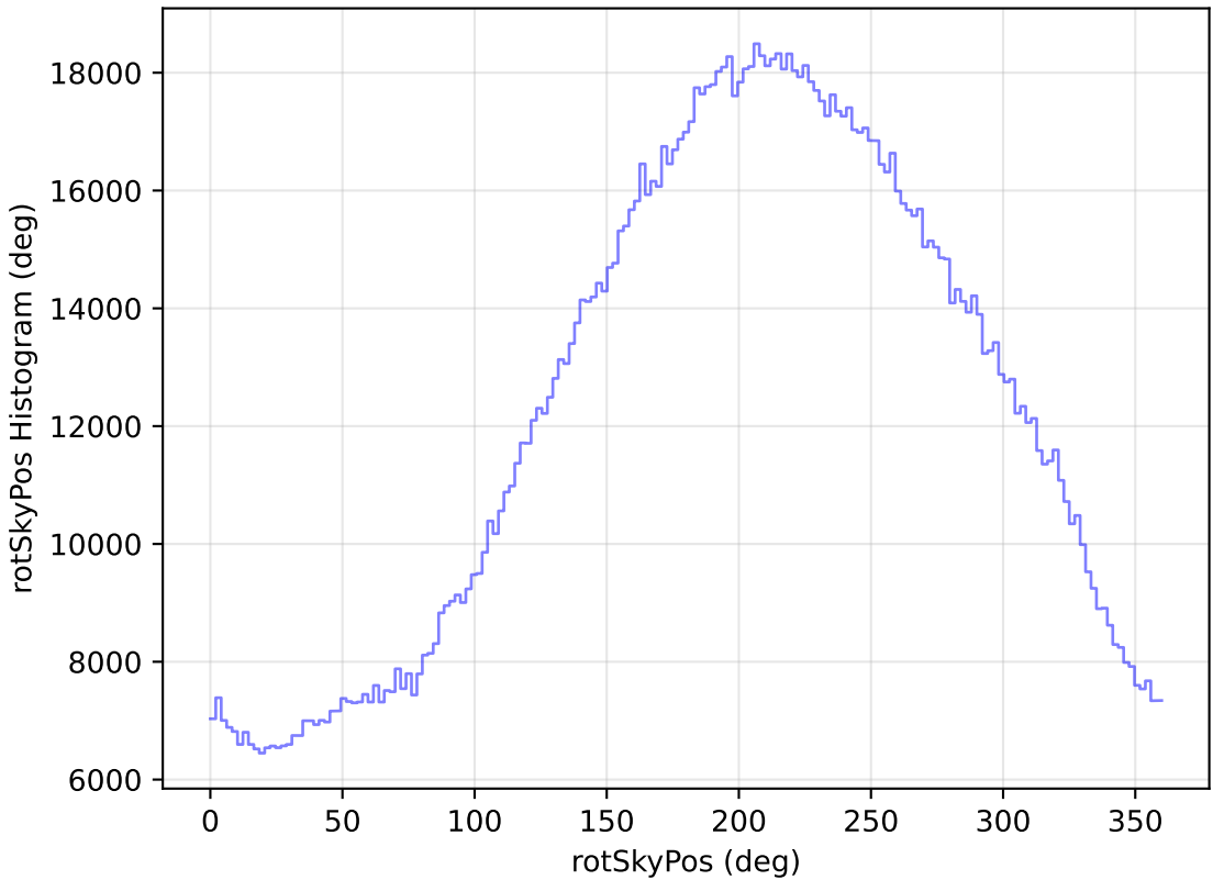
internal_u_expt30_nscale1.1v3.4_10yrs WFD all bands: rotSkyPos Histogram
