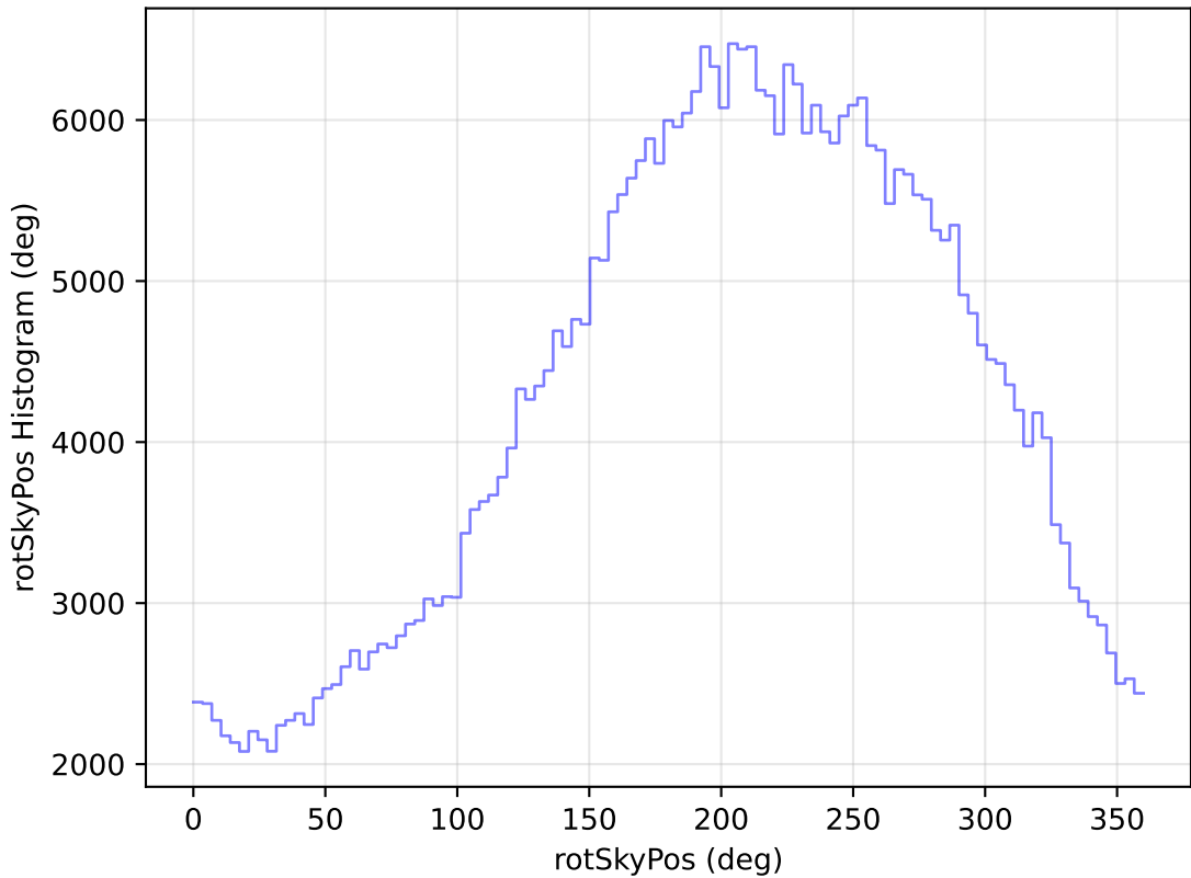
internal_u_expt30_nscale1.1v3.4_10yrs All sky z band: rotSkyPos Histogram
