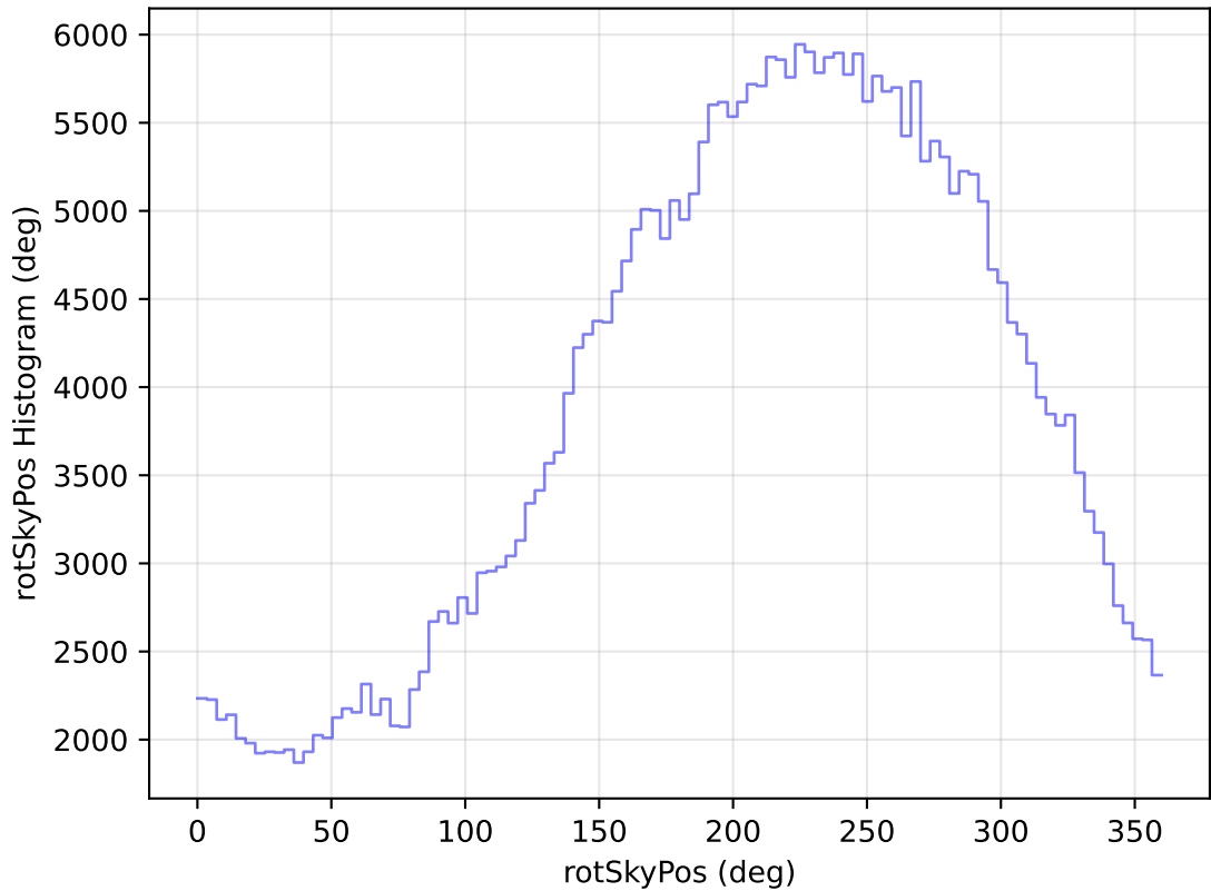
internal_u_expt30_nscale1.1v3.4_10yrs All sky y band: rotSkyPos Histogram
