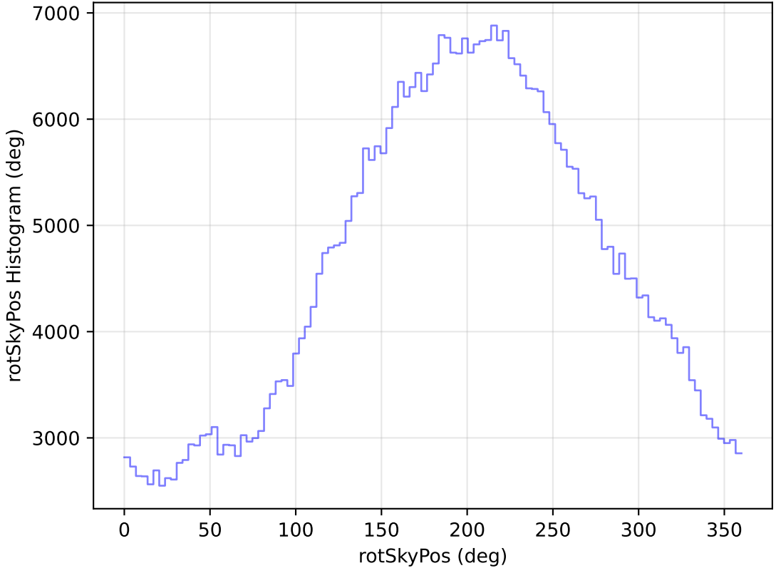
internal_u_expt30_nscale1.1v3.4_10yrs All sky r band: rotSkyPos Histogram
