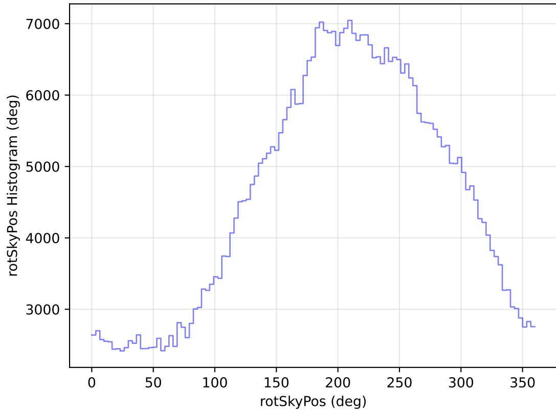
internal_u_expt30_nscale1.1v3.4_10yrs All sky i band: rotSkyPos Histogram
