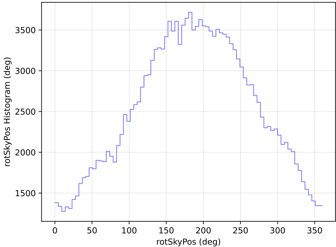
internal_u_expt30_nscale1.1v3.4_10yrs All sky g band: rotSkyPos Histogram
