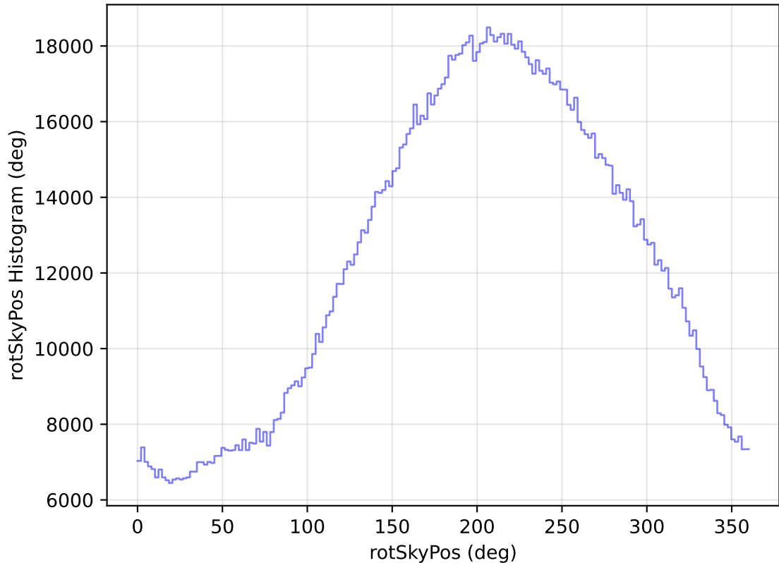
internal_u_expt30_nscale1.1v3.4_10yrs All sky all bands: rotSkyPos Histogram
