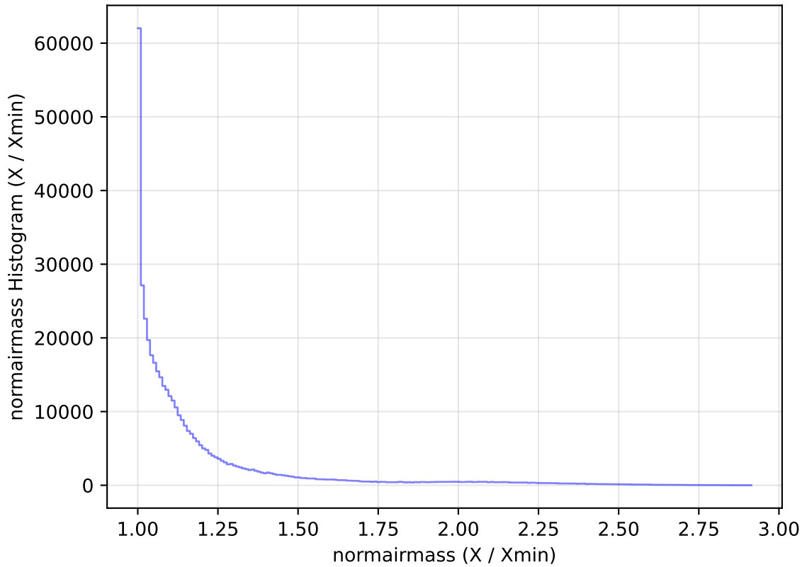
internal_u_expt30_nscale1.1v3.4_10yrs WFD z band: normairmass Histogram
