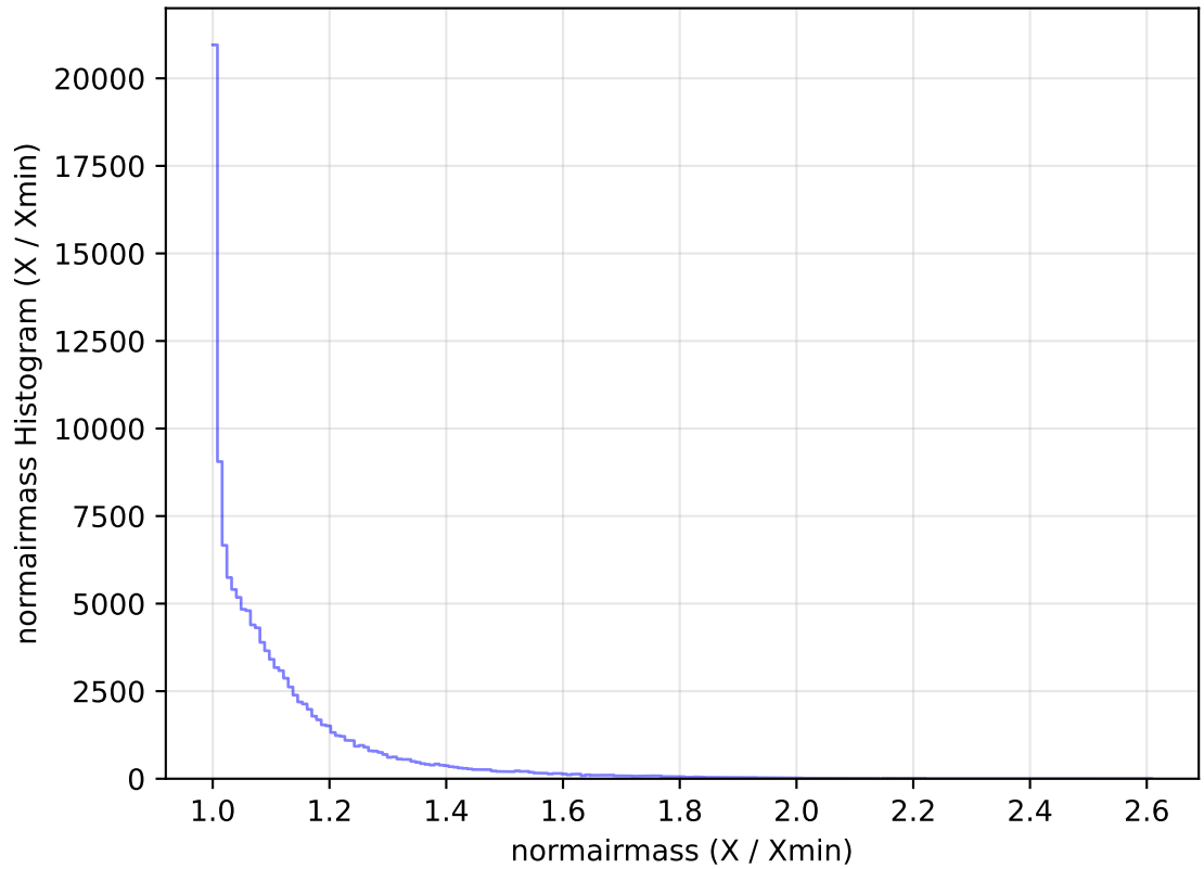
internal_u_expt30_nscale1.1v3.4_10yrs WFD u band: normairmass Histogram
