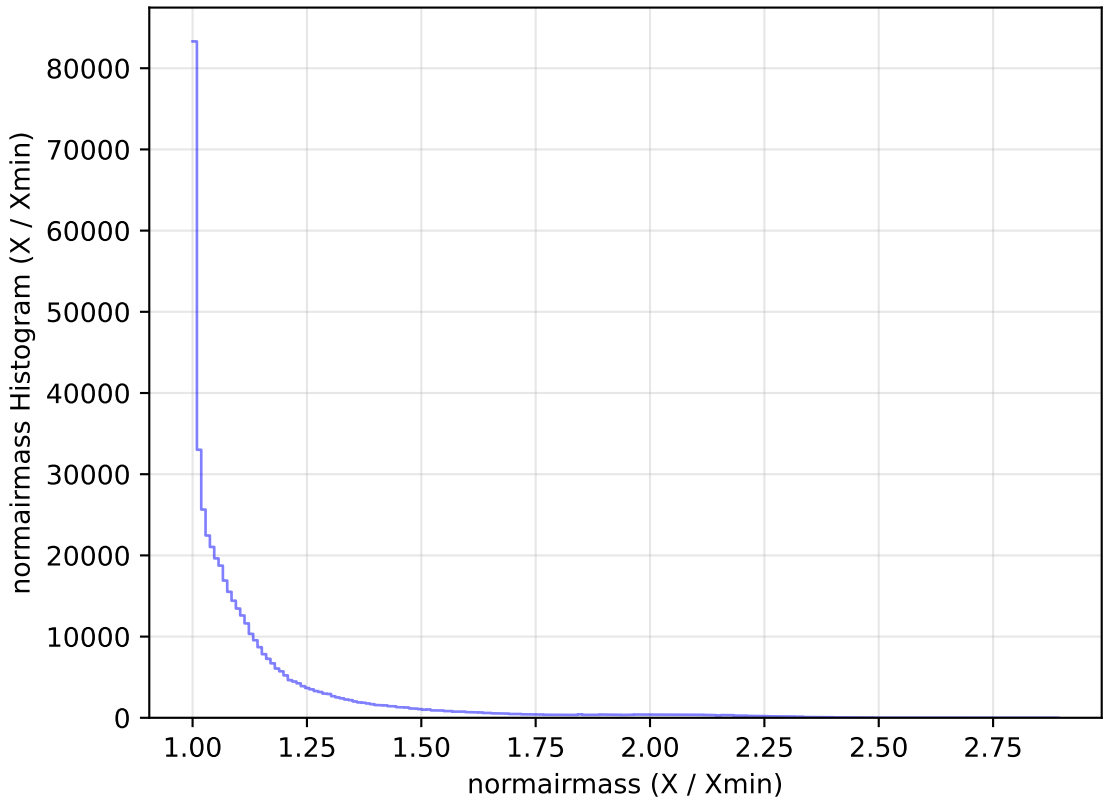
internal_u_expt30_nscale1.1v3.4_10yrs WFD r band: normairmass Histogram
