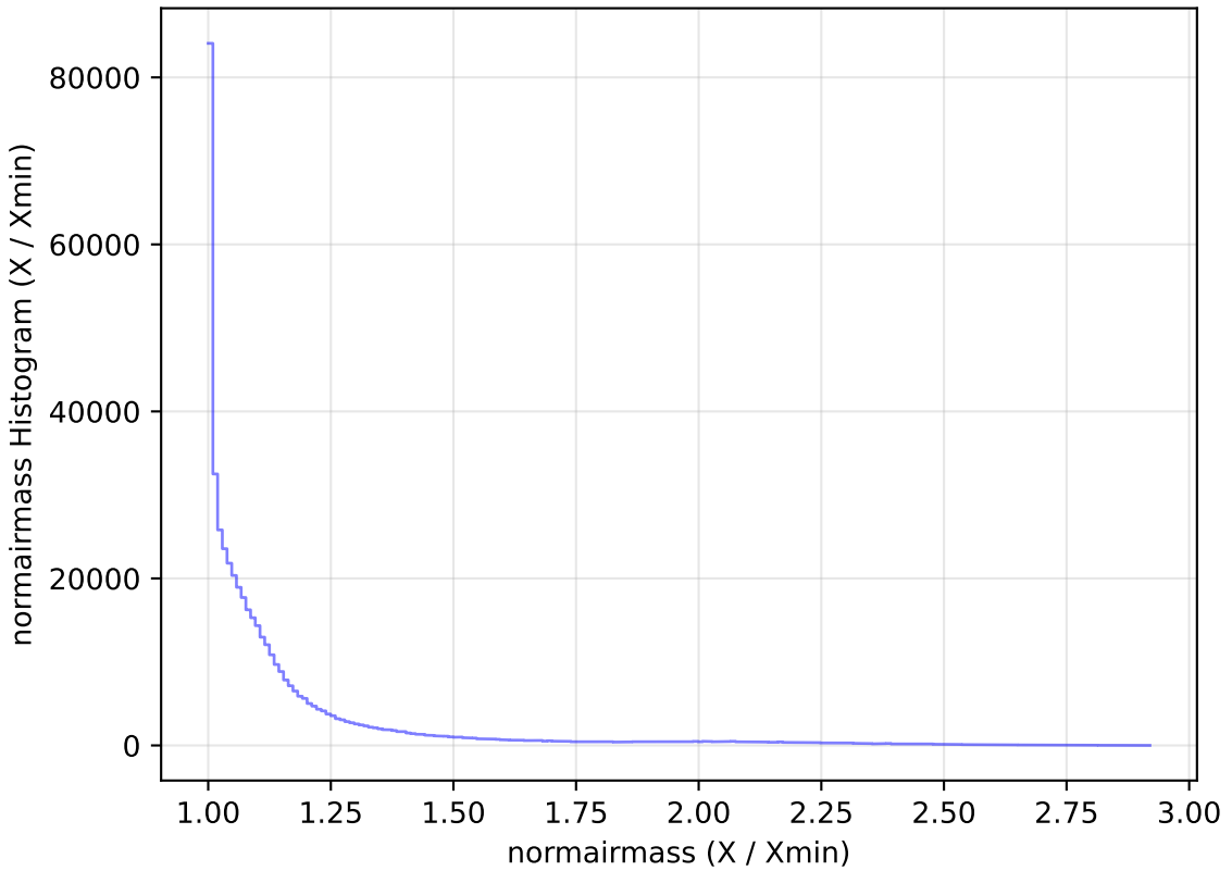
internal_u_expt30_nscale1.1v3.4_10yrs WFD i band: normairmass Histogram
