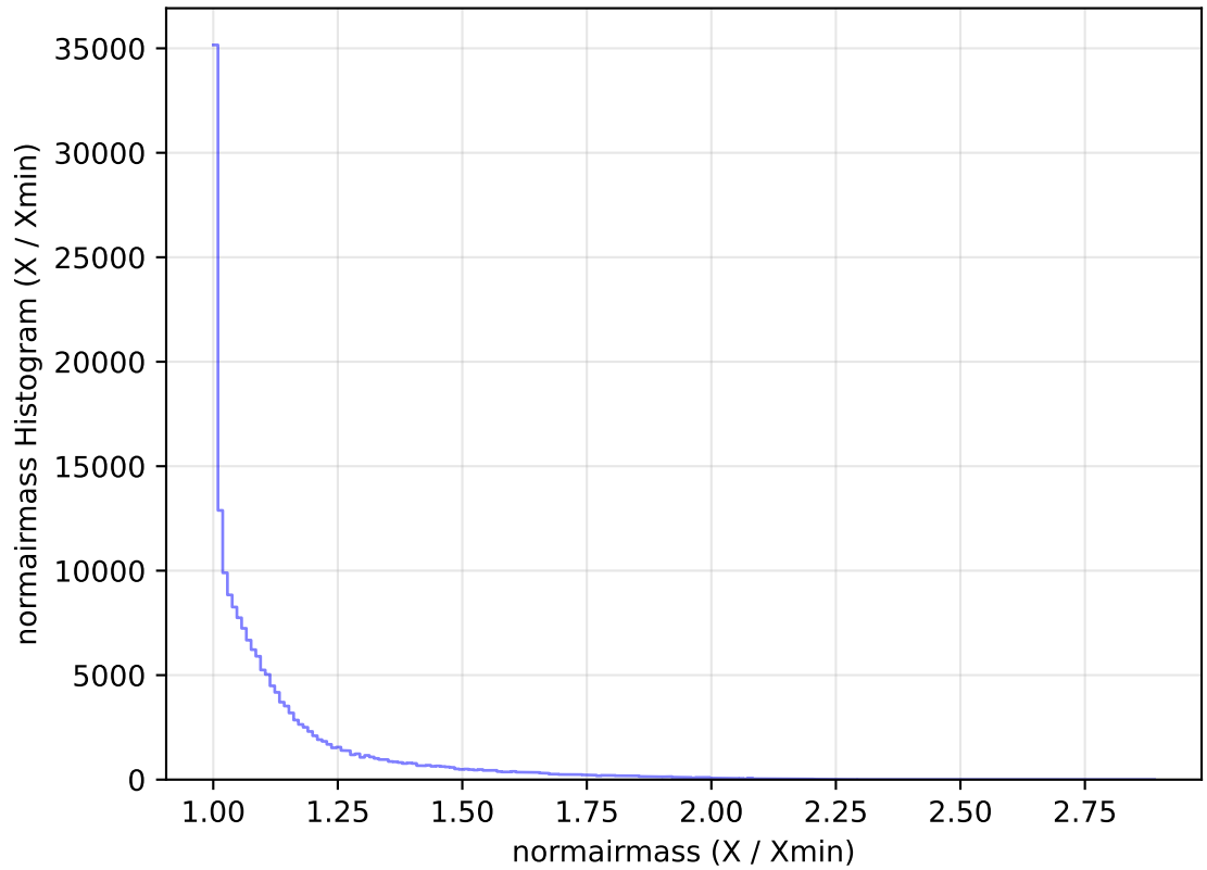
internal_u_expt30_nscale1.1v3.4_10yrs WFD g band: normairmass Histogram
