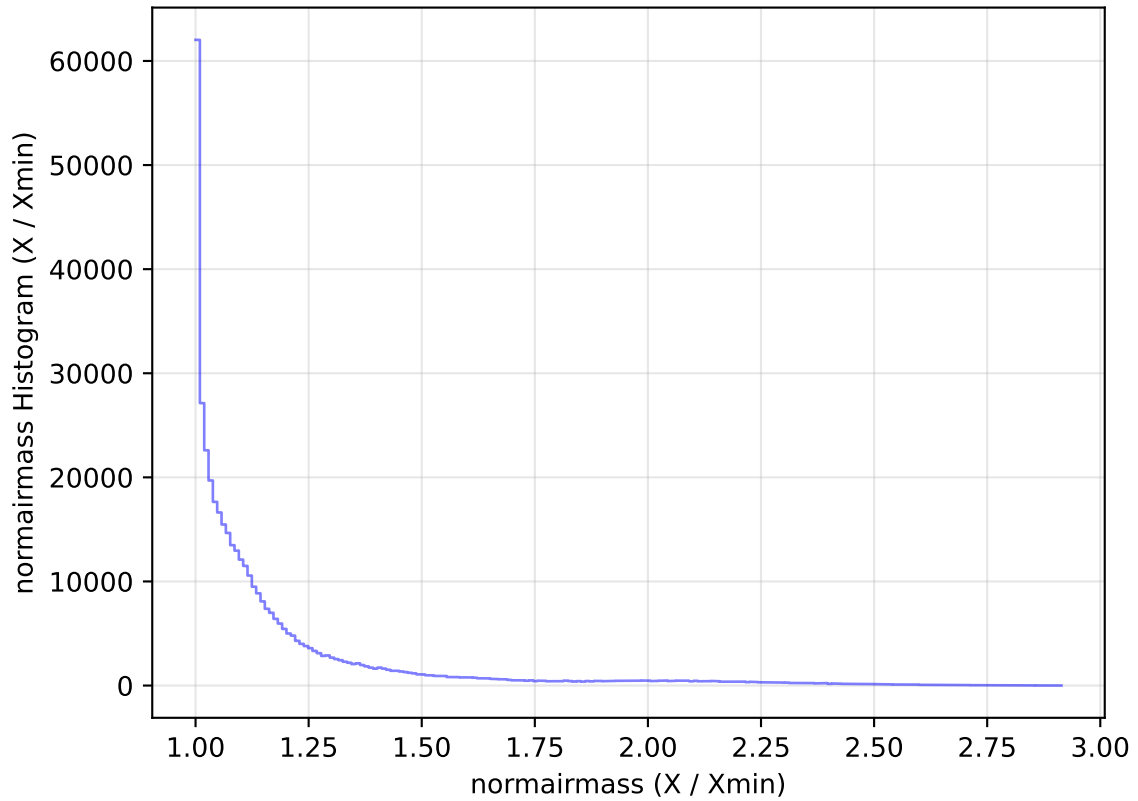
internal_u_expt30_nscale1.1v3.4_10yrs All sky z band: normairmass Histogram
