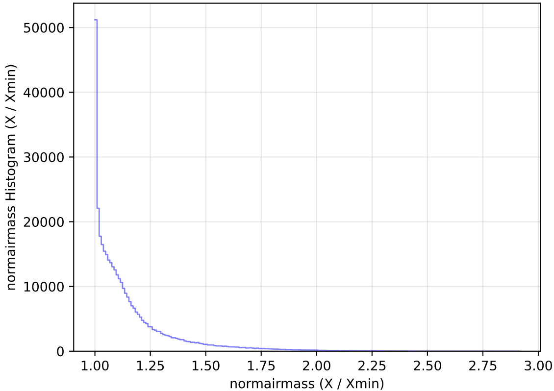
internal_u_expt30_nscale1.1v3.4_10yrs All sky y band: normairmass Histogram
