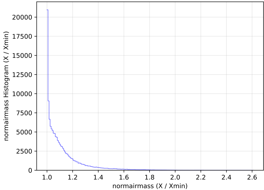
internal_u_expt30_nscale1.1v3.4_10yrs All sky u band: normairmass Histogram
