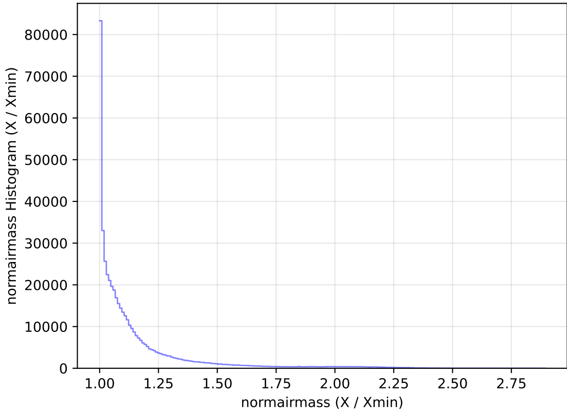
internal_u_expt30_nscale1.1v3.4_10yrs All sky r band: normairmass Histogram
