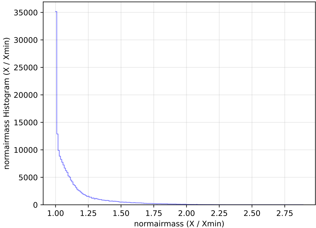
internal_u_expt30_nscale1.1v3.4_10yrs All sky g band: normairmass Histogram
