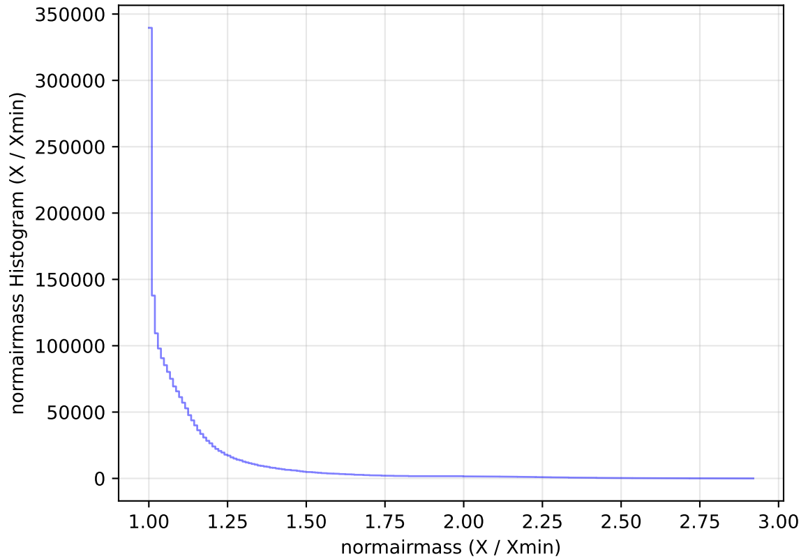
internal_u_expt30_nscale1.1v3.4_10yrs All sky all bands: normairmass Histogram
