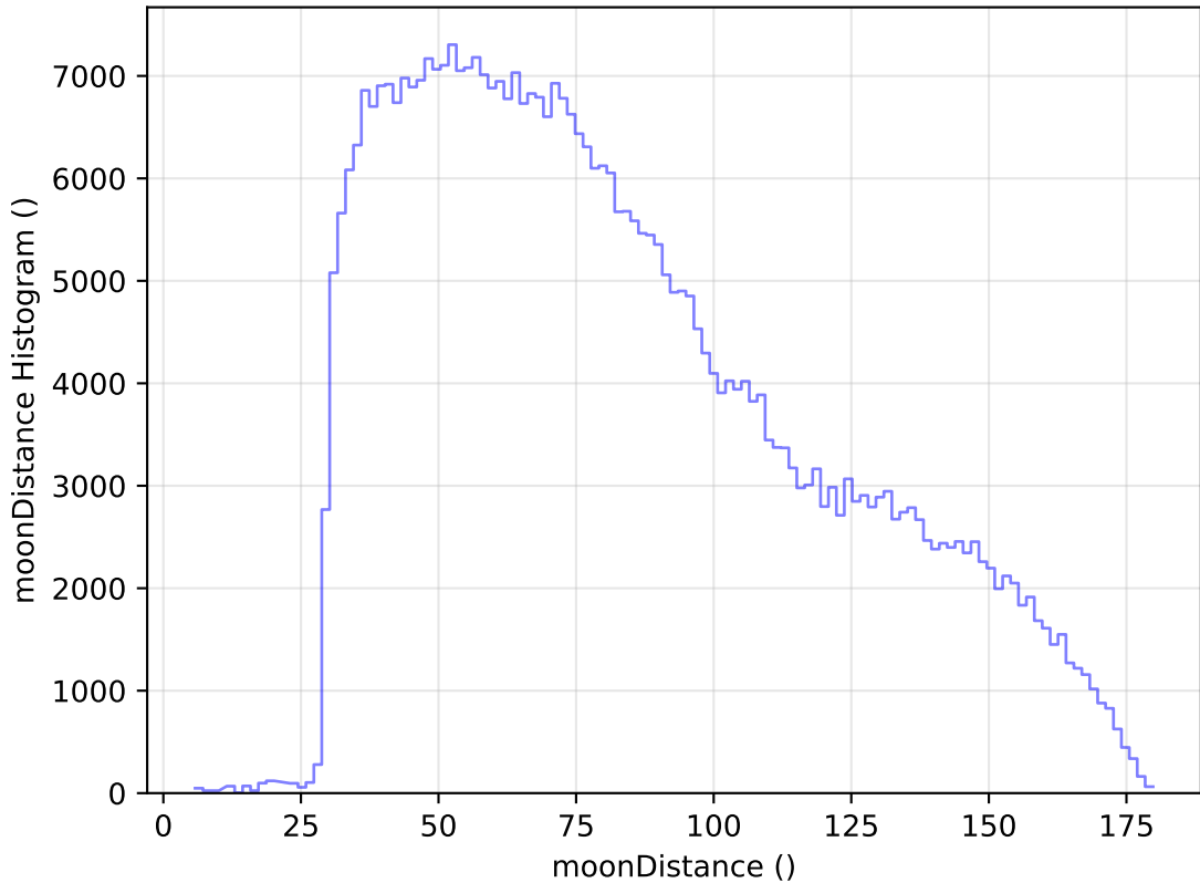
internal_u_expt30_nscale1.1v3.4_10yrs WFD z band: moonDistance Histogram
