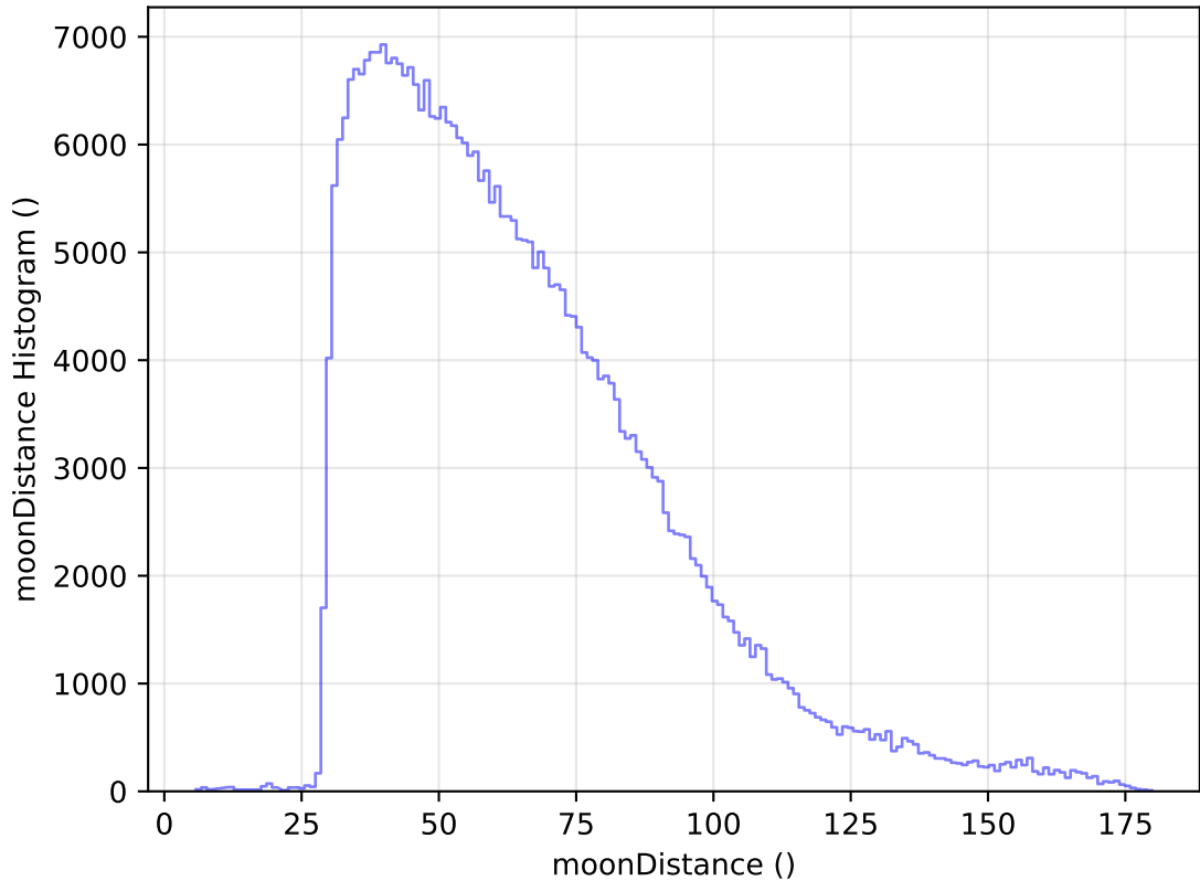
internal_u_expt30_nscale1.1v3.4_10yrs WFD y band: moonDistance Histogram
