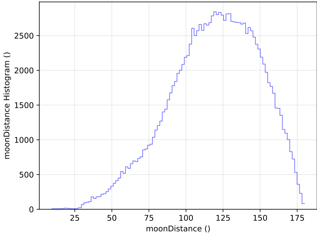
internal_u_expt30_nscale1.1v3.4_10yrs WFD u band: moonDistance Histogram
