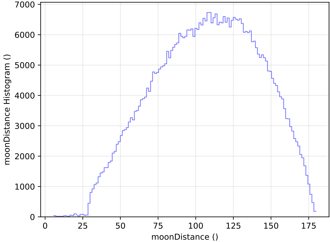
internal_u_expt30_nscale1.1v3.4_10yrs WFD r band: moonDistance Histogram
