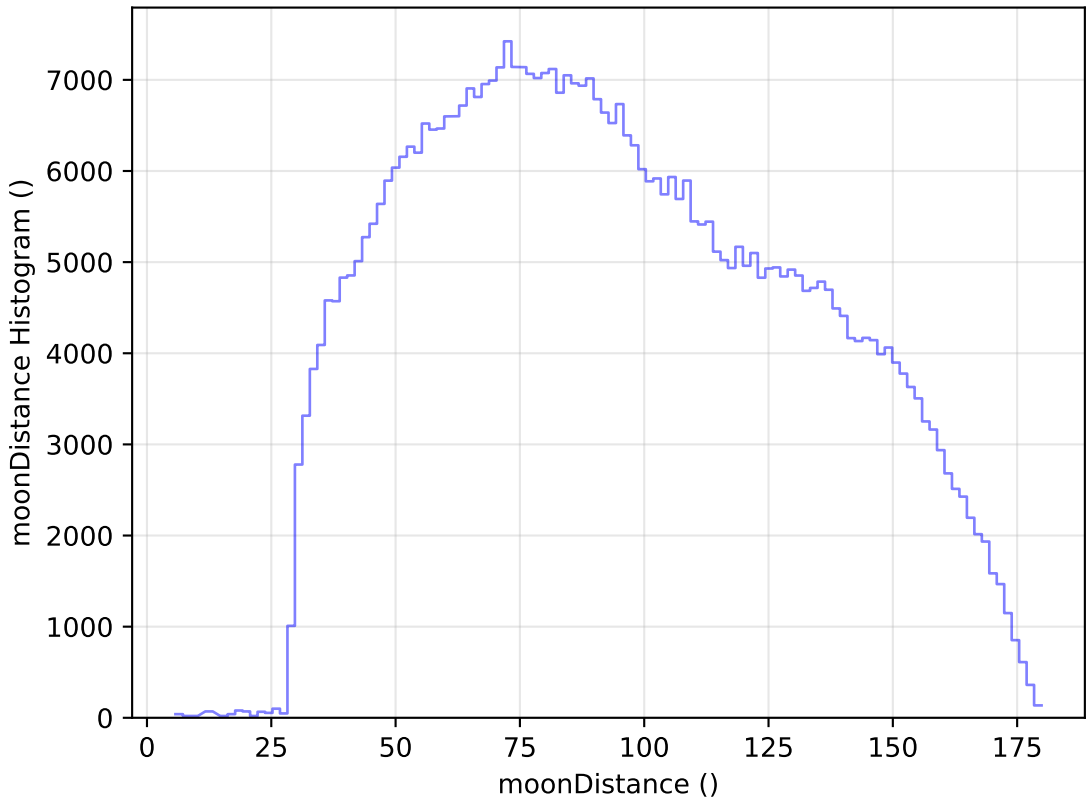
internal_u_expt30_nscale1.1v3.4_10yrs WFD i band: moonDistance Histogram
