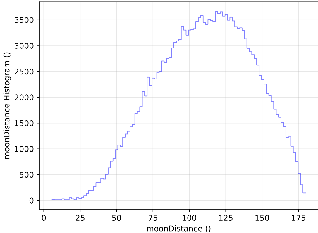
internal_u_expt30_nscale1.1v3.4_10yrs WFD g band: moonDistance Histogram
