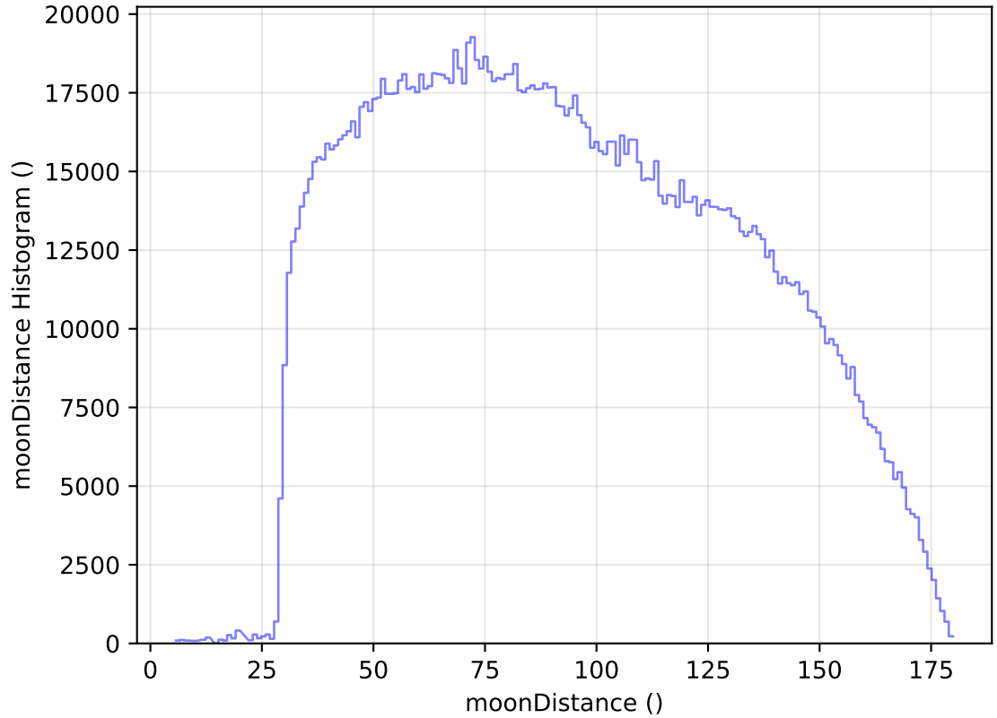
internal_u_expt30_nscale1.1v3.4_10yrs WFD all bands: moonDistance Histogram
