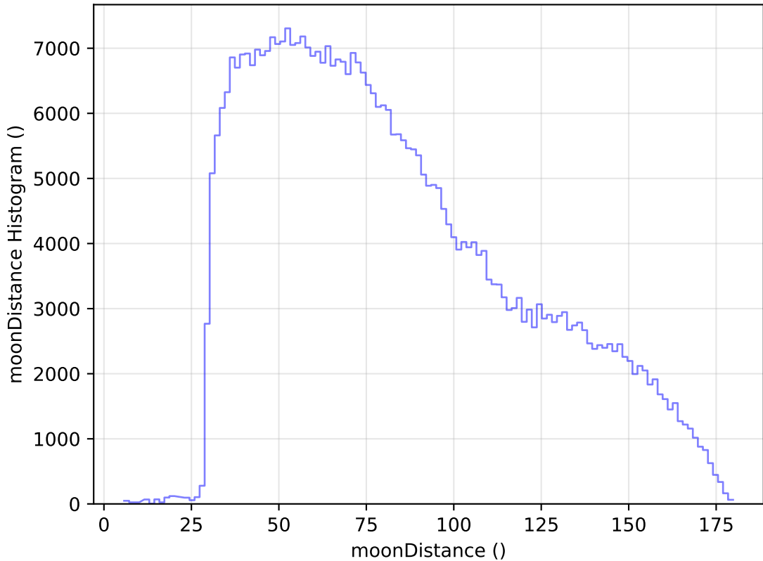
internal_u_expt30_nscale1.1v3.4_10yrs All sky z band: moonDistance Histogram
