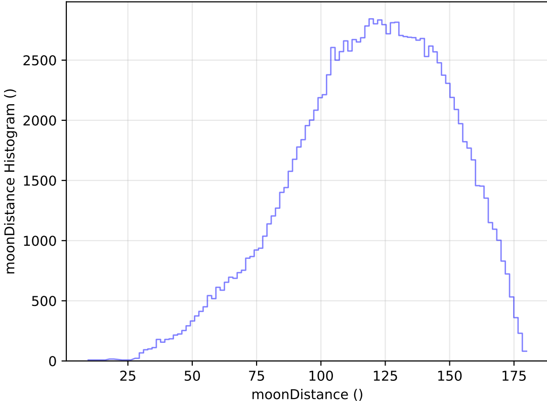
internal_u_expt30_nscale1.1v3.4_10yrs All sky u band: moonDistance Histogram
