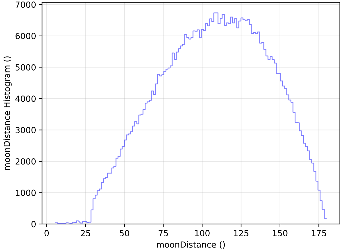
internal_u_expt30_nscale1.1v3.4_10yrs All sky r band: moonDistance Histogram
