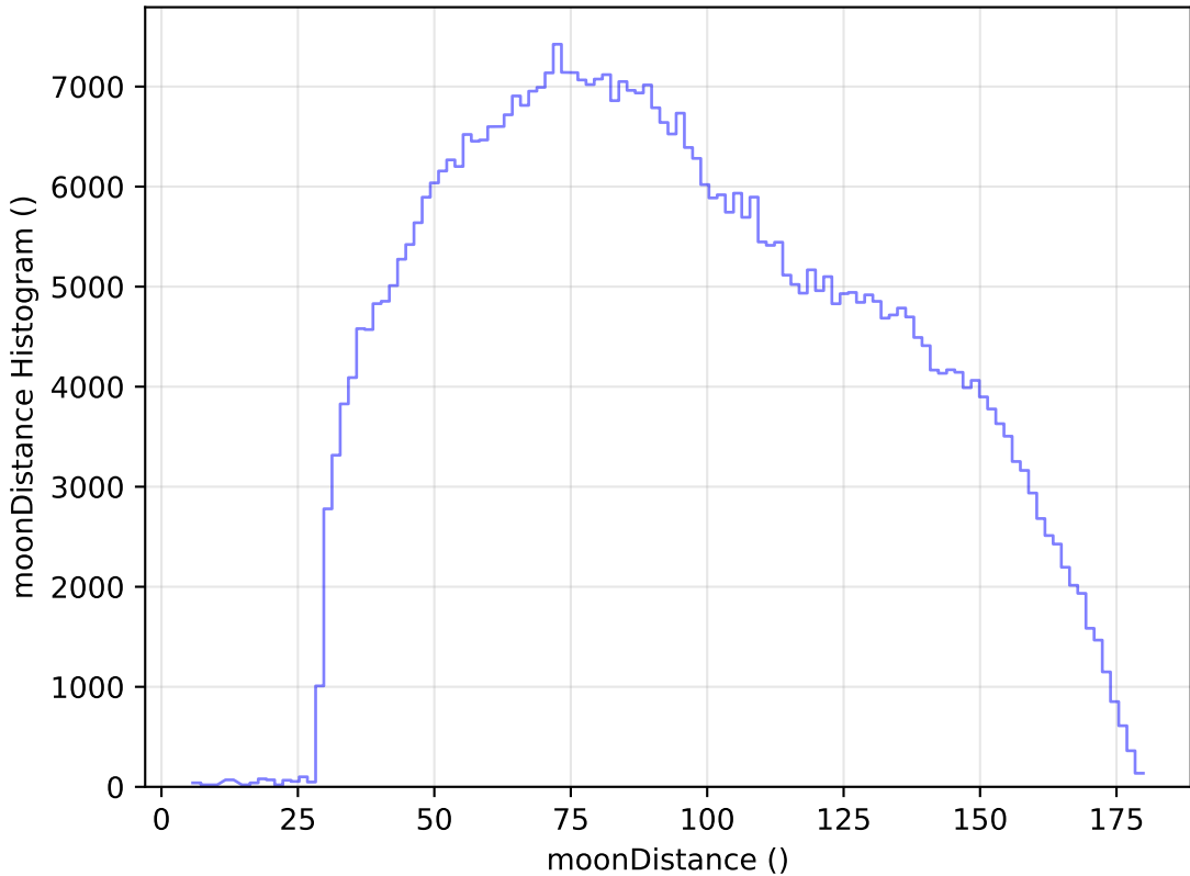
internal_u_expt30_nscale1.1v3.4_10yrs All sky i band: moonDistance Histogram
