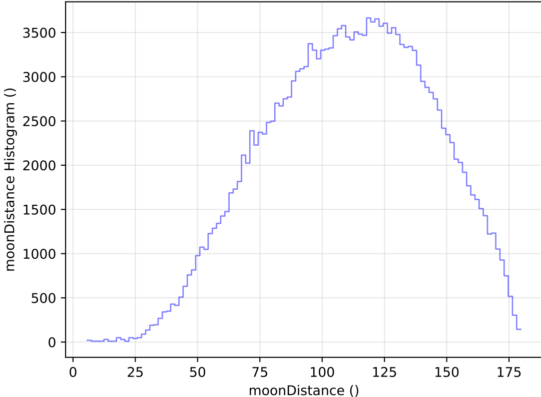
internal_u_expt30_nscale1.1v3.4_10yrs All sky g band: moonDistance Histogram
