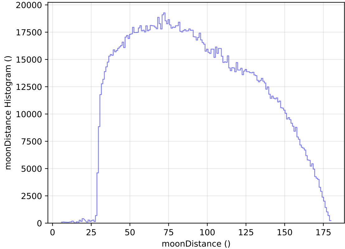
internal_u_expt30_nscale1.1v3.4_10yrs All sky all bands: moonDistance Histogram
