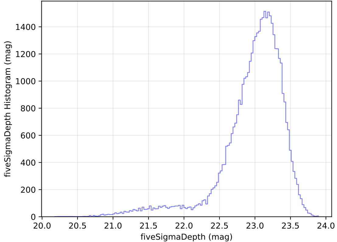
internal_u_expt30_nscale1.1v3.4_10yrs Yr 1 z band: fiveSigmaDepth Histogram
