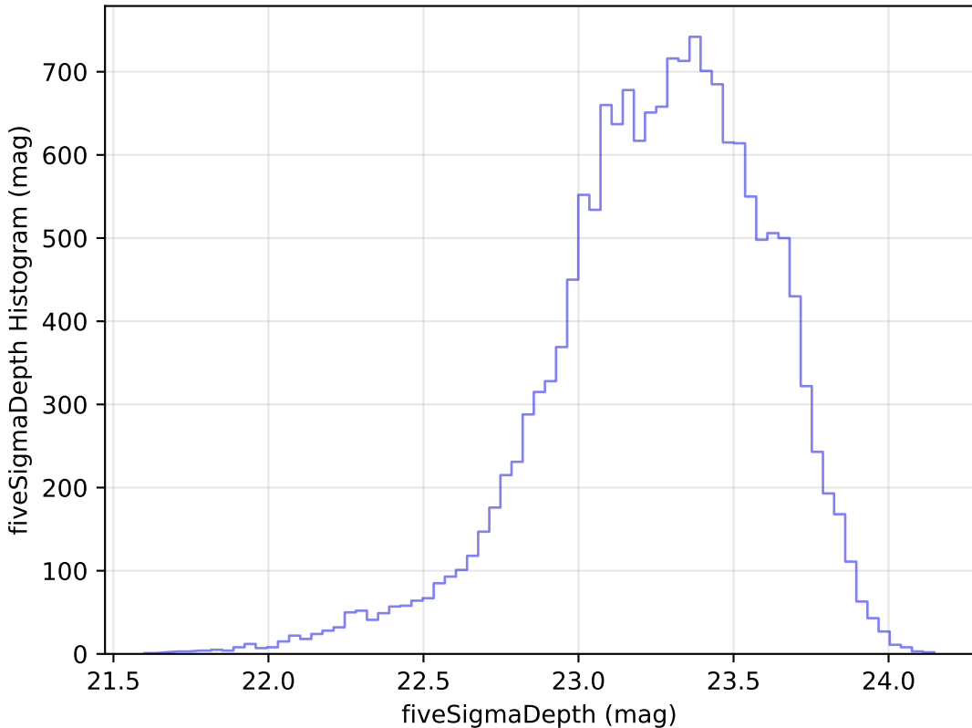
internal_u_expt30_nscale1.1v3.4_10yrs Yr 1 u band: fiveSigmaDepth Histogram
