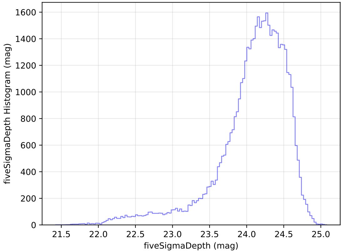
internal_u_expt30_nscale1.1v3.4_10yrs Yr 1 r band: fiveSigmaDepth Histogram
