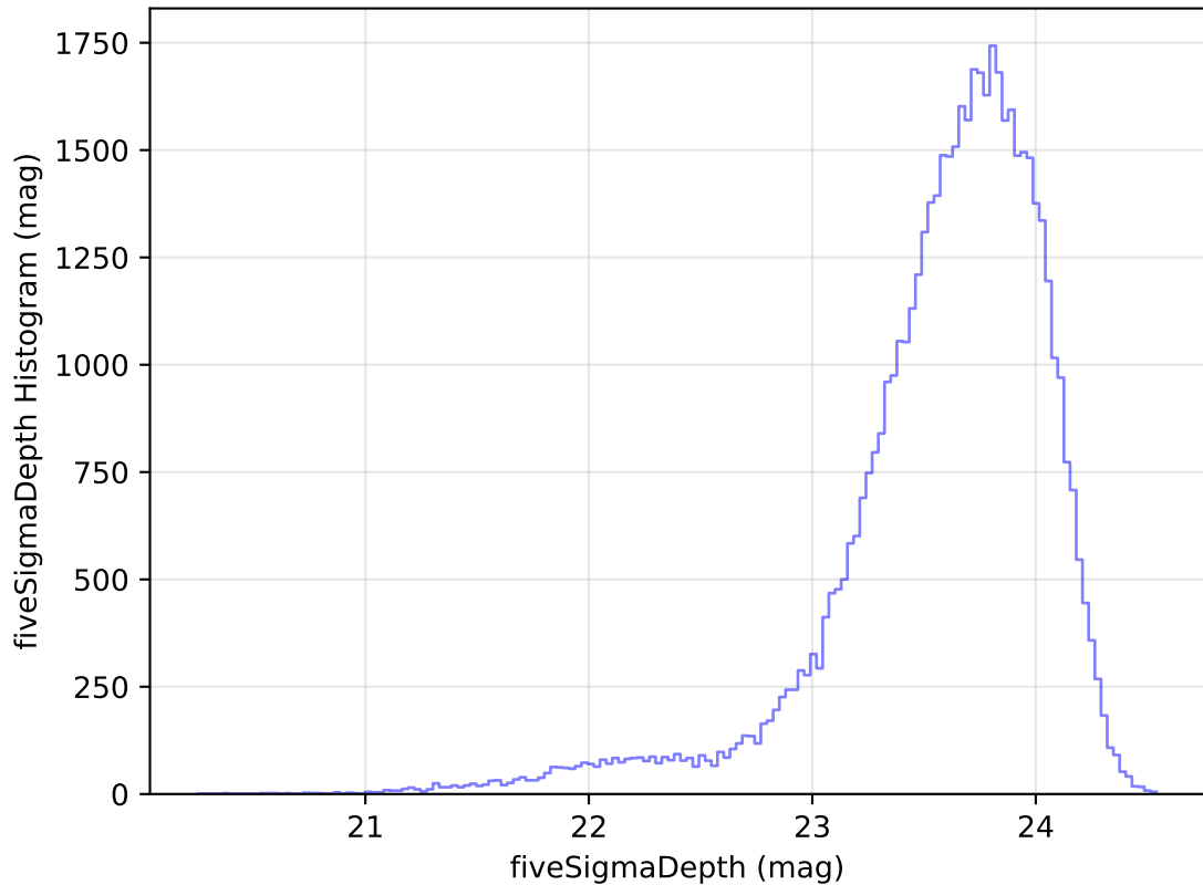
internal_u_expt30_nscale1.1v3.4_10yrs Yr 1 i band: fiveSigmaDepth Histogram
