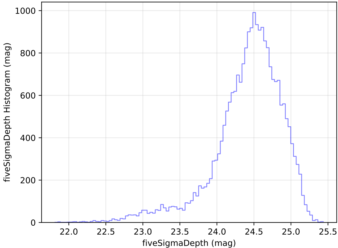
internal_u_expt30_nscale1.1v3.4_10yrs Yr 1 g band: fiveSigmaDepth Histogram
