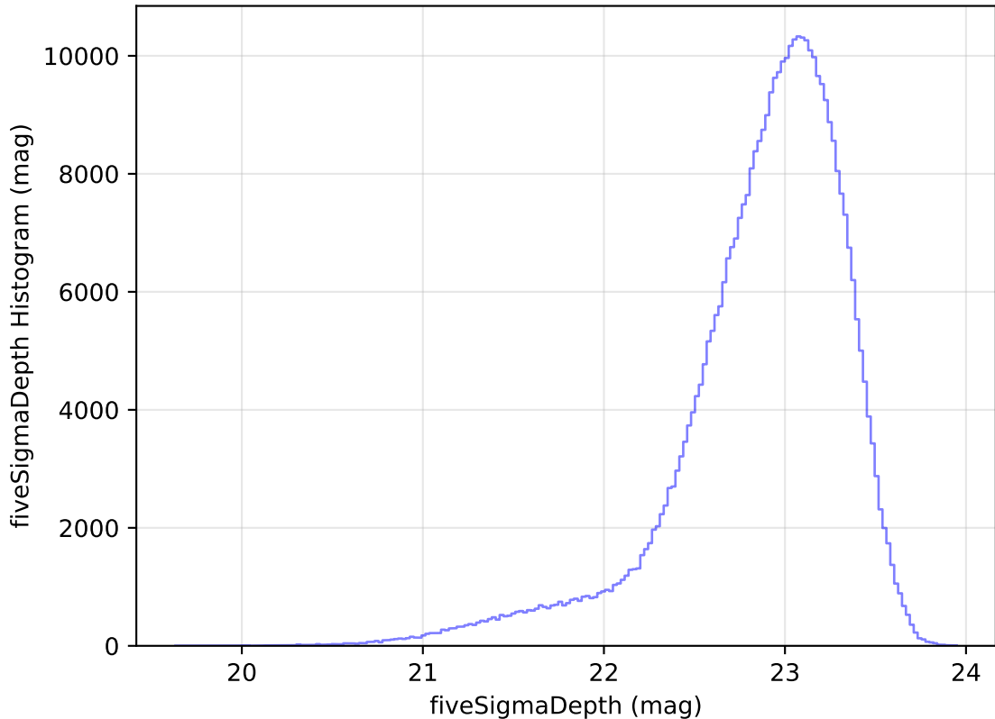
internal_u_expt30_nscale1.1v3.4_10yrs WFD z band: fiveSigmaDepth Histogram
