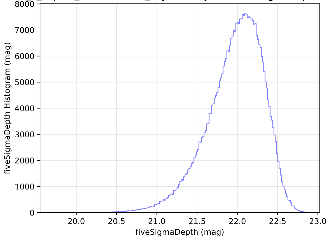
internal_u_expt30_nscale1.1v3.4_10yrs WFD y band: fiveSigmaDepth Histogram
