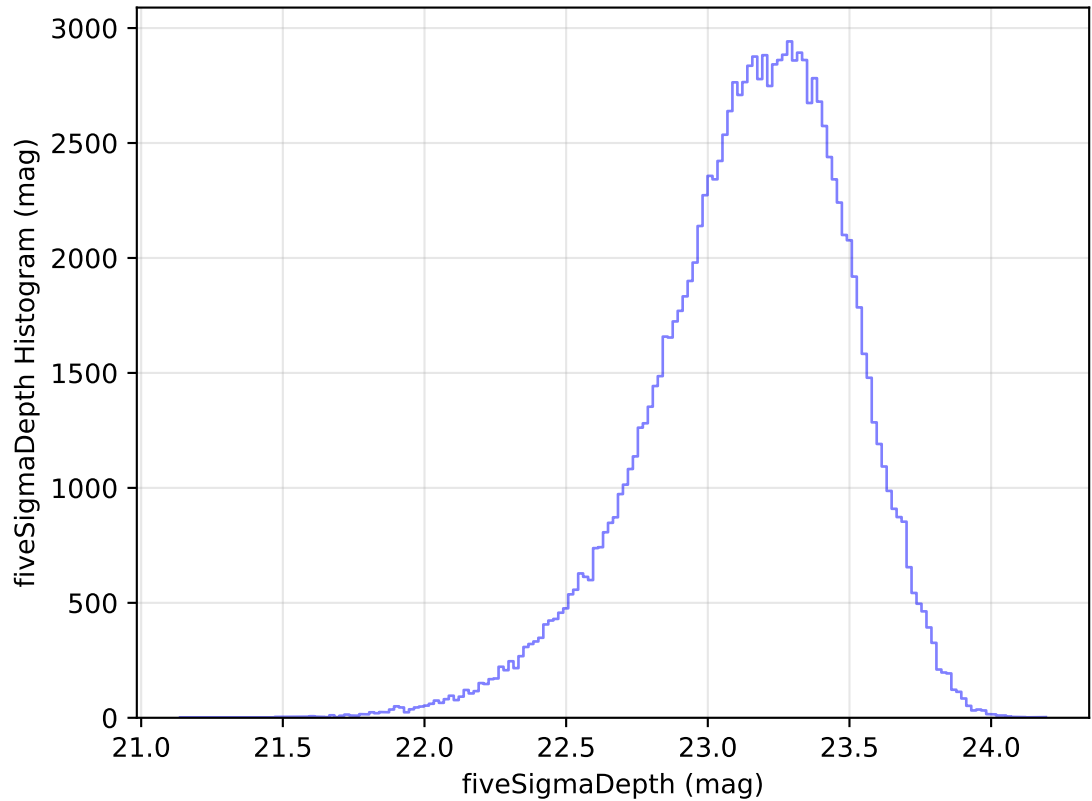
internal_u_expt30_nscale1.1v3.4_10yrs WFD u band: fiveSigmaDepth Histogram
