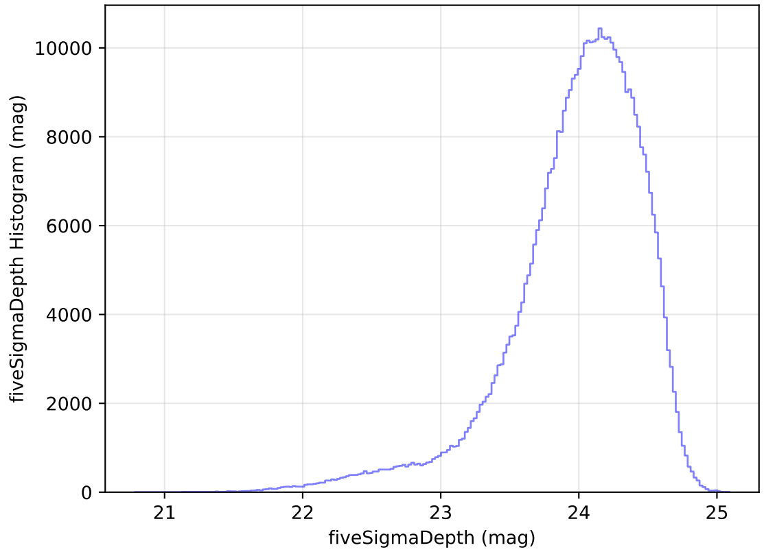
internal_u_expt30_nscale1.1v3.4_10yrs WFD r band: fiveSigmaDepth Histogram
