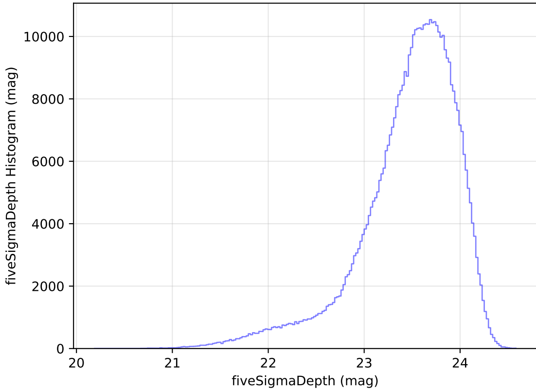
internal_u_expt30_nscale1.1v3.4_10yrs WFD i band: fiveSigmaDepth Histogram
