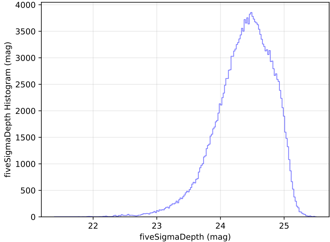
internal_u_expt30_nscale1.1v3.4_10yrs WFD g band: fiveSigmaDepth Histogram
