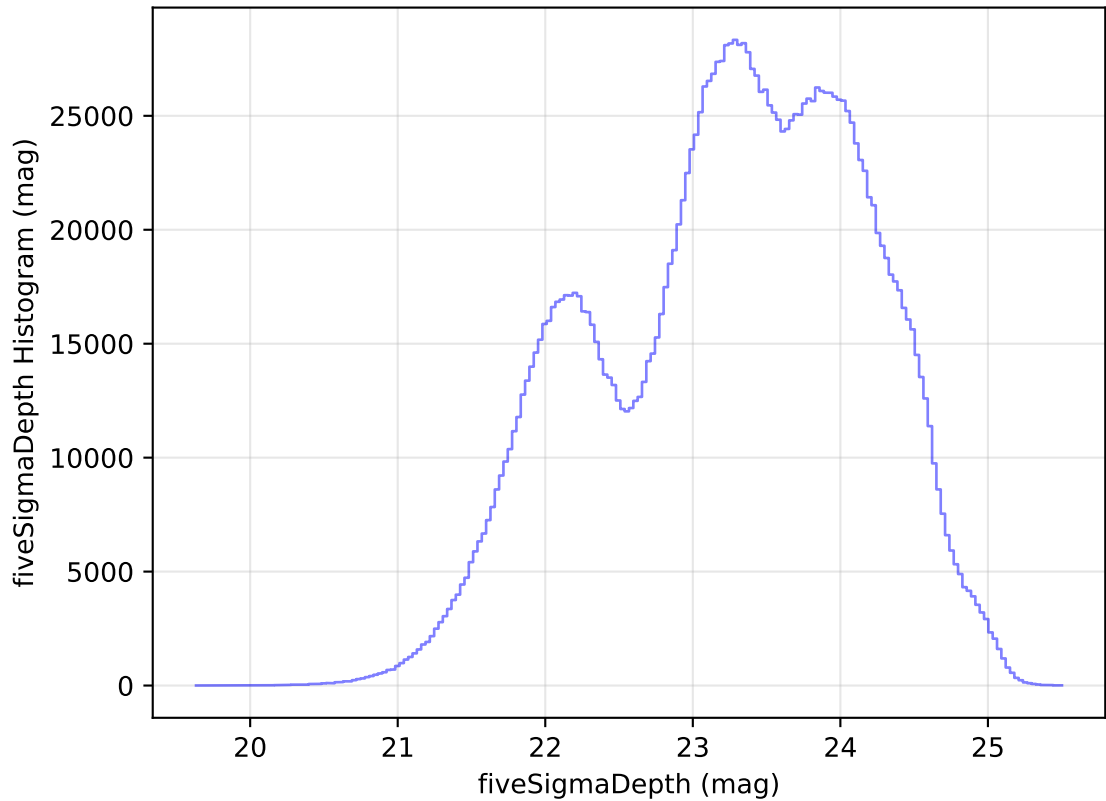
internal_u_expt30_nscale1.1v3.4_10yrs WFD all bands: fiveSigmaDepth Histogram
